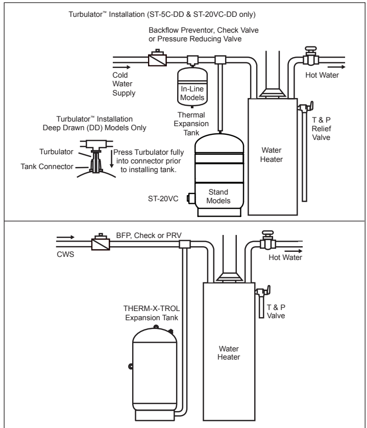
Figure 1. Typical Installation
