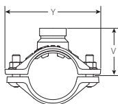
STYLE 922 WITH IGS™ GROOVED OUTLET
