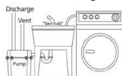
Typical Laundry/Utility Sink Installation
