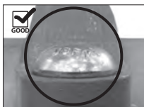
OVAL NECK OF BOLT SEATED PROPERLY
