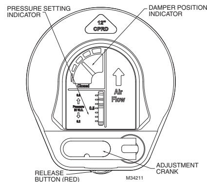
Fig. 4. CPRD regulator
