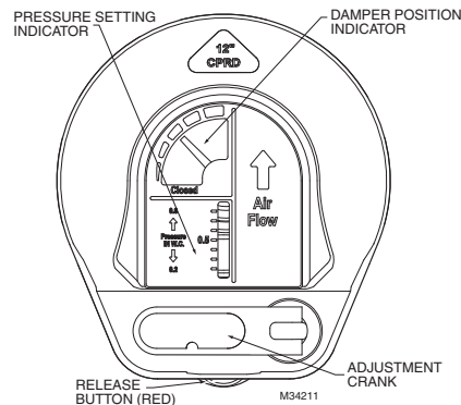
Fig. 4. CPRD regulator
