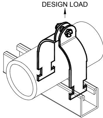
FIGURE 7872 - O.D. Strut Clamp
