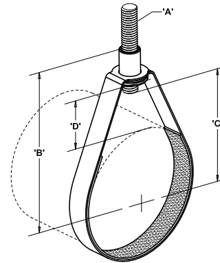
FIGURE 7012 - Felt Lined Adjustable Swivel Ring Hangers
